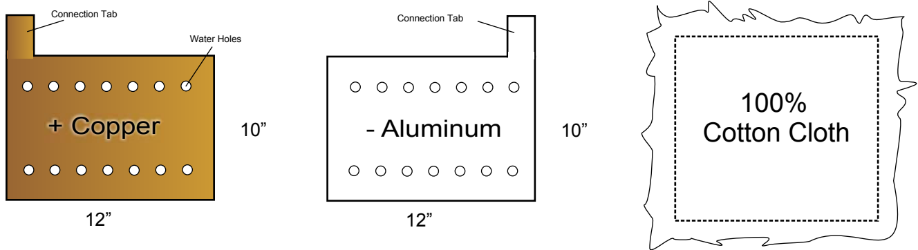
Figure #1 Top View of separate pieces
